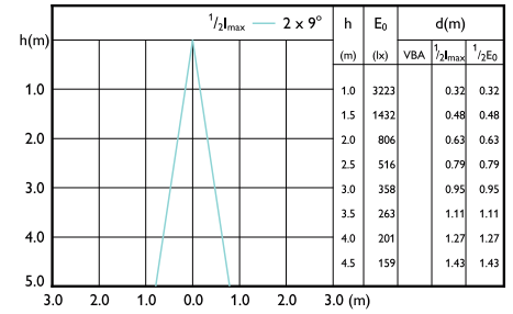
LEDspots MAS IC 7,5W MR16 GU5,3 930 24D-LBP
