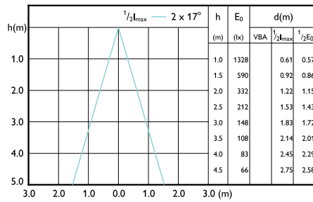
LEDspots MAS IC 7,5W MR16 GU5,3 927 36D-LBP
