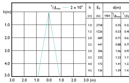
LEDspots MAS IC 6,7W MR16 GU5,3 927 24D-LBP
