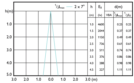
LEDspots MAS IC 6,7W MR16 GU5,3 927 10D-LBP
