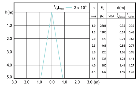
LEDspots MAS IC 6,7W MR16 GU5,3 930 24D-LBP
