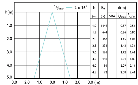
LEDspots MAS IC 6,7W MR16 GU5,3 930 36D-LBP
