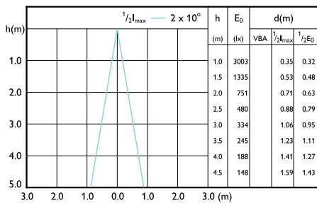
LEDspots MAS IC 6,7W MR16 GU5,3 940 24D-LBP
