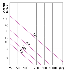
LEDspots MAS IC 7,5W MR16 GU5,3 940 24D-LA2
