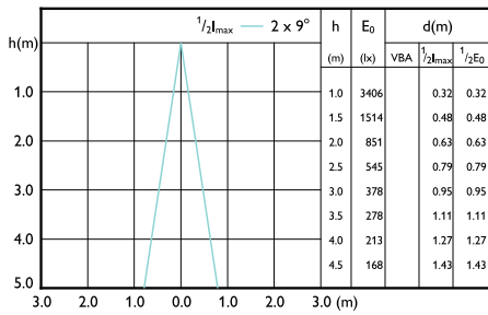
LEDspots MAS IC 7,5W MR16 GU5,3 940 24D-LBP
