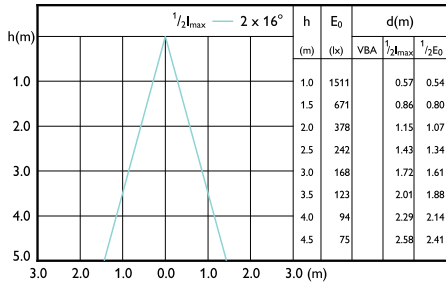
LEDspots MAS IC 6,7W MR16 GU5,3 940 36D-LBP
