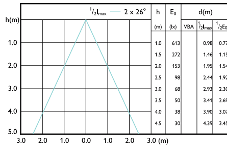
LEDspots MAS IC 6,7W MR16 GU5,3 930 60D-LBP
