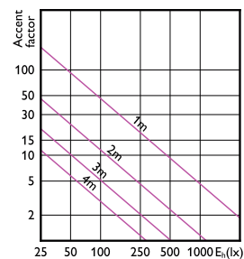
LEDspots MAS IC 6,7W MR16 GU5,3 927 10D-LA2
