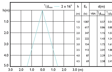
LEDspots MAS IC 6,7W MR16 GU5,3 927 36D-LBP
