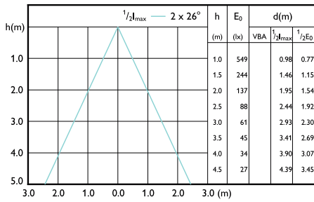
LEDspots MAS IC 6,7W MR16 GU5,3 927 60D-LBP
