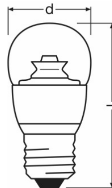
PARATHOM CL P 40 ADV 6 W/827 E27 CS
