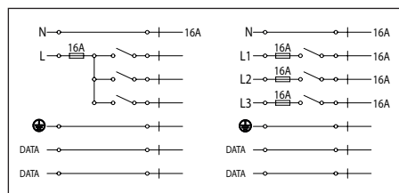
Schaltplan Electrical scheme
