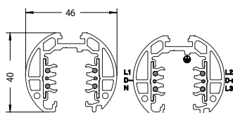
Round version (...-ST15) Round version (...-ST15)
