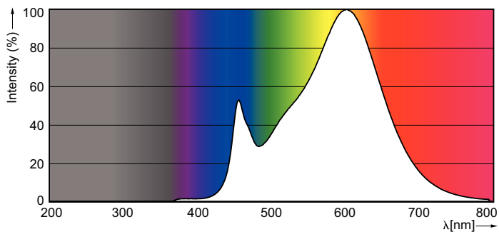
CorePro LEDspotMV 35W GU10 830 36D CLA
