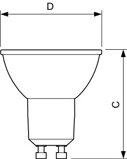
GU10 230V4W-35W 265lm 25D 4000K GU10 Dim
