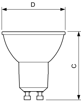
GU10 7.5-80W 650lm 2700K GU10 D 15khrs
