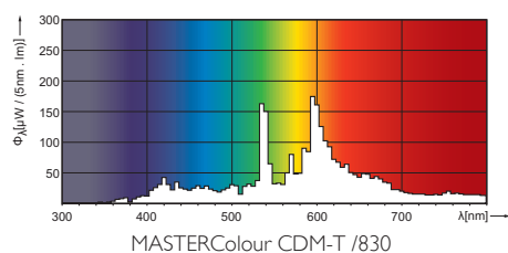
MASTERColour CDM-T /830
