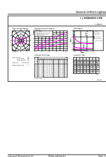
LEDbulb MAS 5,9W G120 E27 927 CL-GUL
